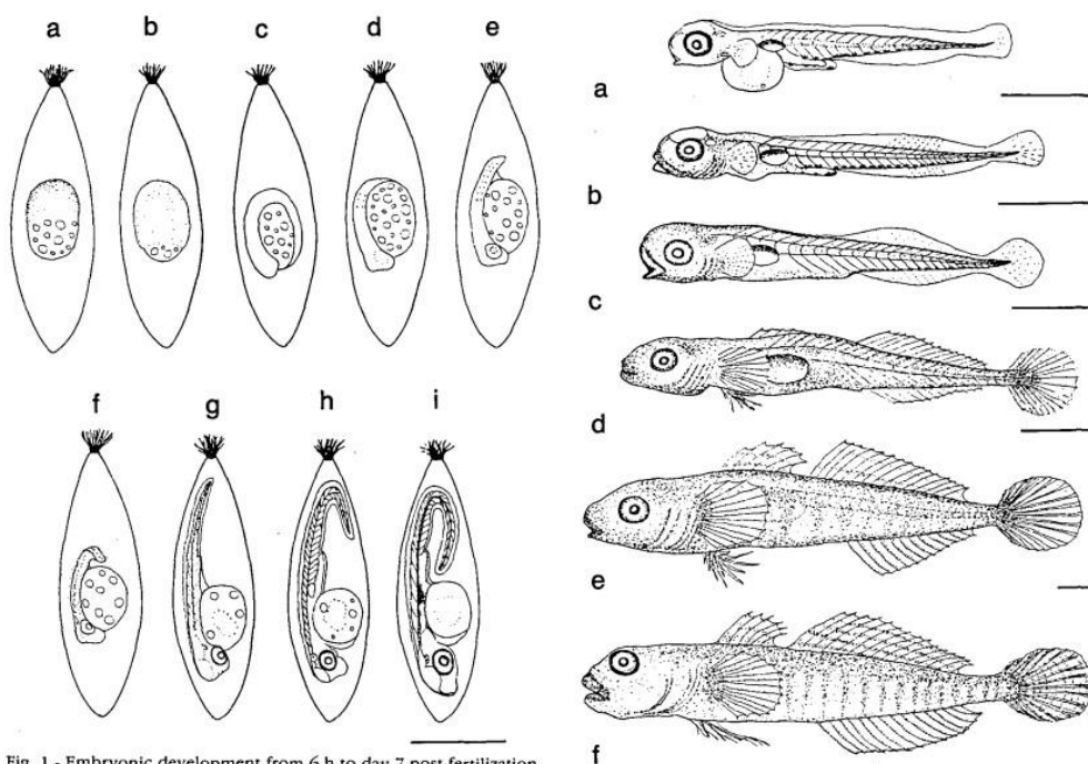
Fig. 1 - Embryonic development from 6 h to day 7 post-fertilization (PF). a) 6 h PF, blastula stage; b) 24 h PF, closing blastopore stage; c) 36 h PF, head fold stage; d) 48 h PF, 3 somite and optic vesicle stage; e) 60 h PF, 8 somite and tail bud stage; f) 80 h PF, auditory vesicles, primordial fin and 26 somite stage; g) 106 h PF, pigmented eye stage; h) 128 h PF, swimbladder pigmented stage; i) 152 h PF, developed pectoral fins, heart beating, 28 somite stage. Scale bar: 1 mm.
